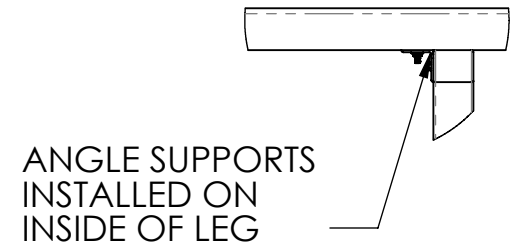
③ ASSEMBLY DETAIL
